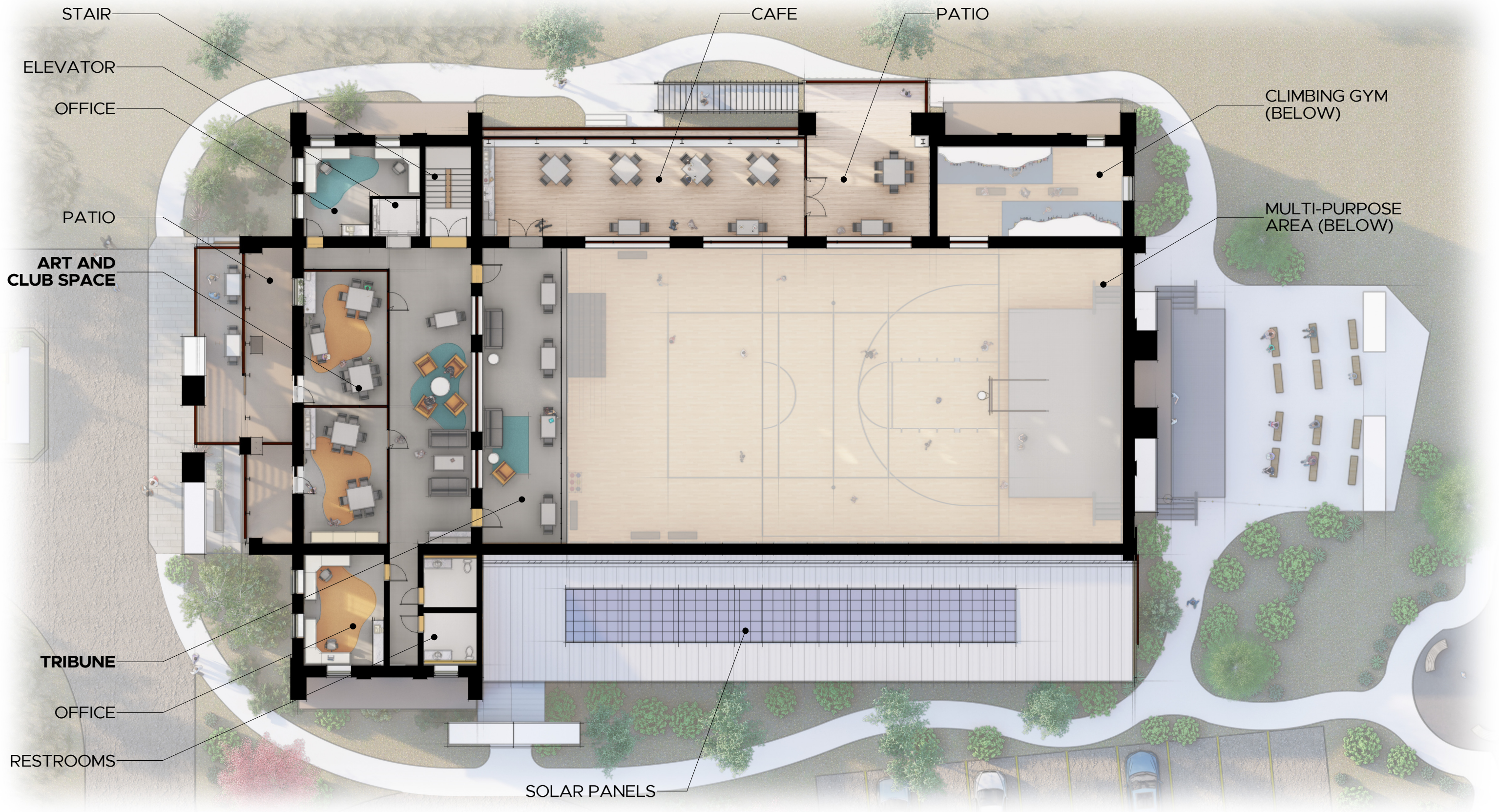
SOLDATSKÉ CULTURAL CENTER PROPOSED SECOND FLOOR PLAN
